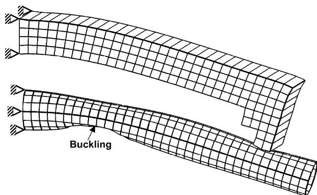
Fig. 6. An example of the nano-valve configuration at the onset of SWCNT buckling.
